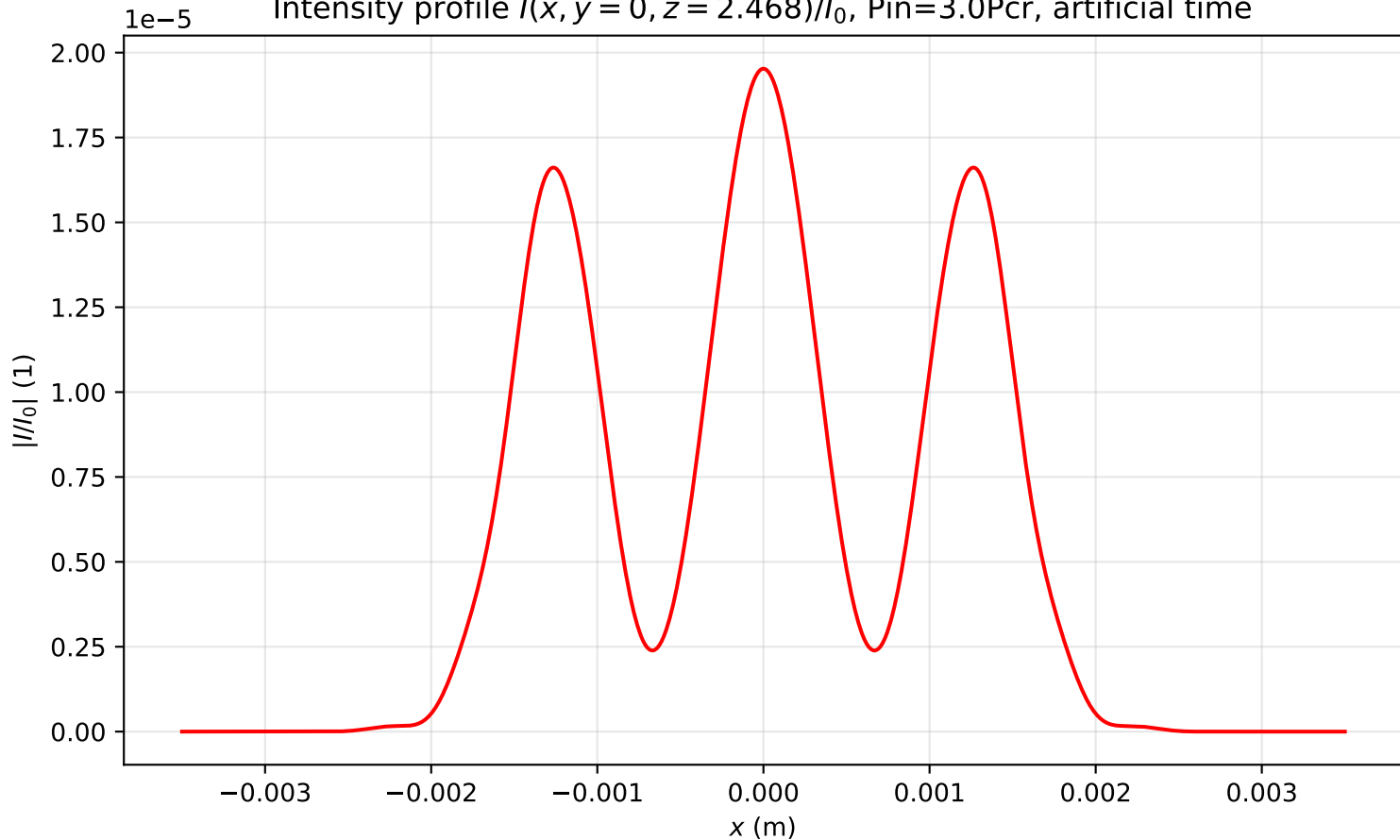
Intensity profile I(x, y = 0, z = 2.468)/I_0 , P_{in}=3.0P_{cr} , artificial time
